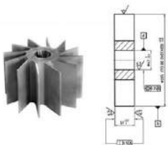
Pump Impeller Casting Process: Precision Casting Material: AISI316, AISI304, CF8M,
