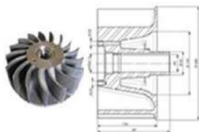
Vacuum Pump Impeller Casting Process: Precision Casting Material: AISI316, AISI304, CF8M
