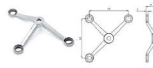
Material: SS304, SS316 Finish: Mirror, Satin L: 160, 200, 220, 260, 300
