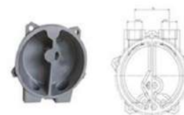
Pump Casing Casting Process: Precision Casting Standard: AISI316, AISI304, CF8M
