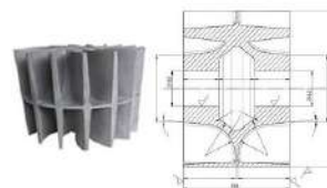
Stainless Steel Pump Impeller Casting Process: investment casting Material: AISI316, AISI304, CF8M
