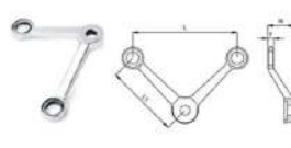
Material: SS304, SS316 Finish: Mirror, Satin L: 160, 200, 220, 260, 300
