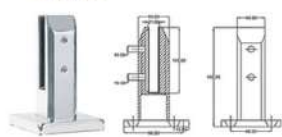
HB-001 Material: SS304, SS316, Duplex 2205 Finish: Mirror, Satin
