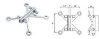
Material: SS304, SS316 Finish: Mirror, Satin L: 160, 200, 220, 260, 300
