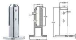
HB-002 Material: SS304, SS316, Duplex 2205 Finish: Mirror, Satin
